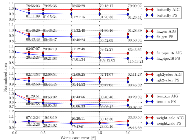
Figure 2. Normalized area in dependence of the specified error bound. The labels show the average runtimes of the approximation process in the format hours:minutes:seconds.
