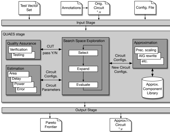
Figure 1. Architecture of the CIRCA approximation framework.
